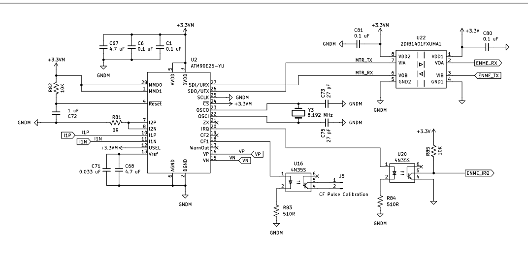
Single Phase Metering
