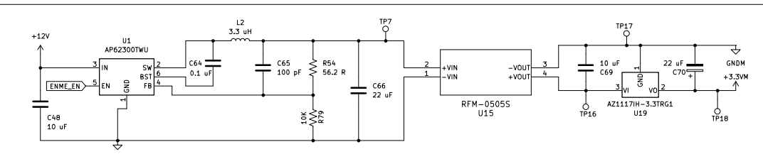
Power Supply for Metering
