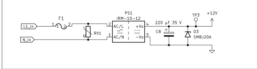
AC-&gt;DC converter
