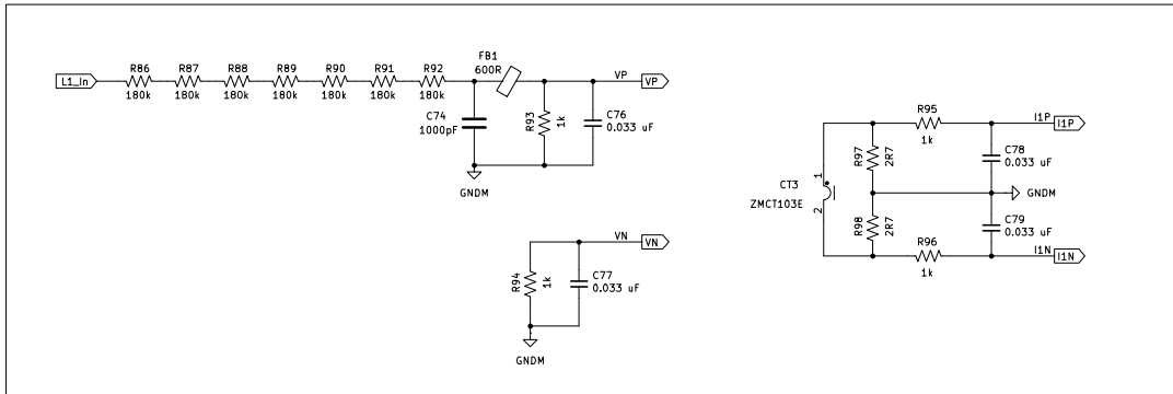
Single Phase Metering
