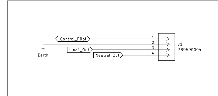
Output Connectors
