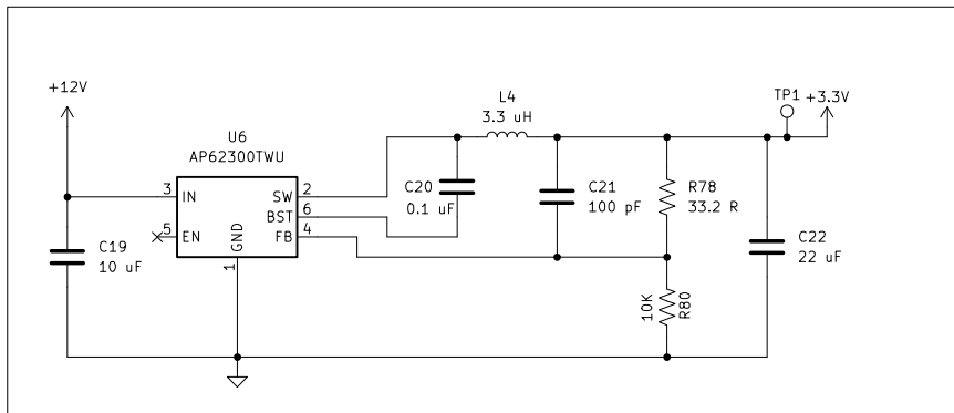
Power Supply MCU
