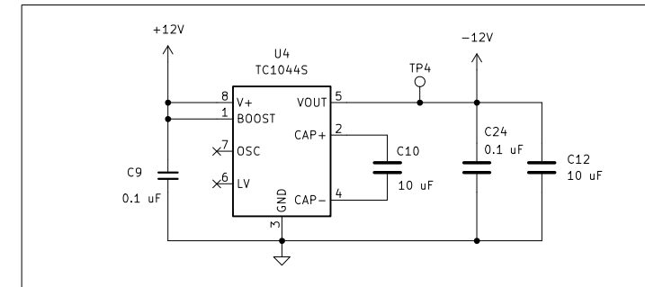
-12V Power regulator for CP-PP
